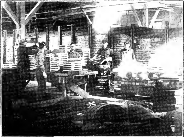
The Tunnel Kiln Furnace Shifts Unloading Respirator Carbon, Filling and Striking Trays and loading Crude Carbon
